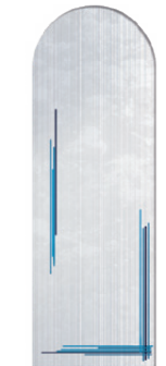
Fusion V8.5
